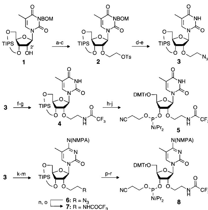
Scheme 1. Synthesis of protected 2'-aminoethoxy phosphoramidites thymidine ( 5 ) and C5-methylcytidine ( 8 ): a) BrCH 2 CO 2 Me (5 equiv), NaH (2.2 equiv), DMF, 1.5 h, –5 °C, 98 %; b) LiBH 4 (4 equiv), MeOH/THF (2/8), 1.5 h, 5 °C, 84 %; c) TsCl (1.5 equiv), NEt 3 (1.6 equiv), DMAP (10 wt %), CH 2 Cl 2 , 8 h, 22 °C, 89 %; d) H 2 , Pd/C (20 wt %), HCl (0.02 equiv), THF/MeOH (1/1), 7 h, 22 °C, 88 %; e) NaN 3 (3 equiv), DMF, 3 h, 65 °C, 92 %; f) SnCl 2 (3.5 equiv), MeOH, 1 d, 22 °C, 70 %; g) (CF 3 CO) 2 O (1.2 equiv), pyridine, 2 h, 22 °C, 57 %; h) TBAF (2.1 equiv), THF, 15 min, 22 °C, 100 %; i) DMTTrCl (1.2 equiv), pyridine, 16 h, 22 °C, 85 %; j) (iPr 2 N) 2 -POCH 2 CH 2 CN (2.2 equiv), diisopropylammonium tetrazolide (2.4 equiv), CH 2 Cl 2 , 1 h, 22 °C, 85 %; k) triazole (22.5 equiv), POCl 3 (2.5 equiv), NEt 3 (23 equiv), CH 3 CN/CH 2 Cl 2 (1/1), 3 h, 22 °C; l) concd NH 3 (aq)/dioxane (1/1), 1 h, 22 °C, 84 % over two steps; m) N -methyl-2,2-dimethoxypyrrolidine (1.8 equiv), pyridine, 3 h, 22 °C, 95 %; n) H 2 , Pd/C (10 wt %), MeOH/THF (1/1), 3 h, 22 °C; o) CF 3 COOEt (10 equiv), NEt 3 (7 equiv), MeOH, 1 h, 22 °C, 96 % over two steps; p) TBAF (1.0 equiv), THF, 1 h, 22 °C, 100 %; q) DMTTrCl (1.2 equiv), pyridine, 1 h, 22 °C, 85 %; r) (iPr) 2 N 2 -POCH 2 CH 2 CN (2.2 equiv), diisopropylammonium tetrazolide (2.4 equiv), CH 2 Cl 2 , 2 h, 40 °C, 87 %. TIPS = 1,1,3,3-tetraisopropylidisiloxane, BOM = benzyloxymethyl, N(NMPA) = N -methylpyrrolidinamidine, DMF = N,N -dimethylformamide, THF = tetrahydrofuran, DMAP = 4-dimethylaminopyridine, TBAF = tetra- n -butylammonium fluoride, DMTTr = 4,4'-dimethoxytriphenylmethyl, Ts = toluene-4-sulfonyl.
